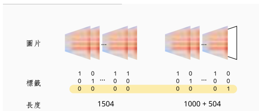
Figure 5: 頻譜圖長度補齊
