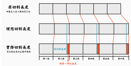
Figure 3: 切割長度計算
